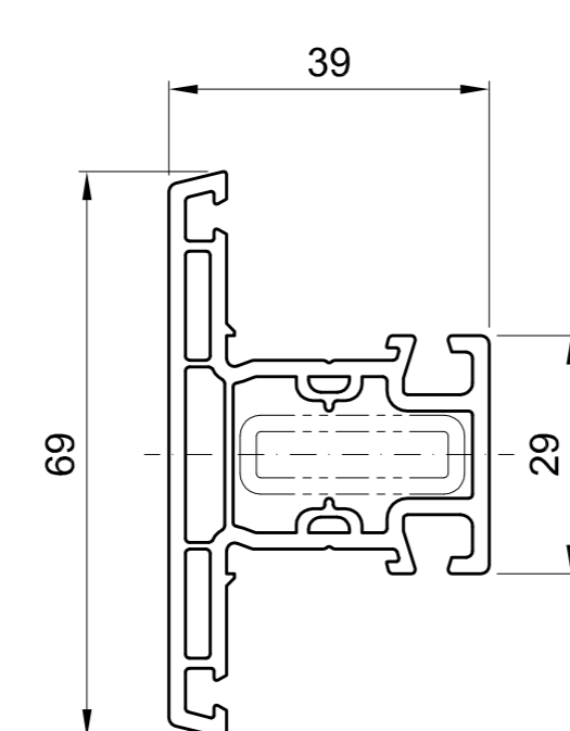
652 010 Steel tube 27,4x9,6: 655 010
