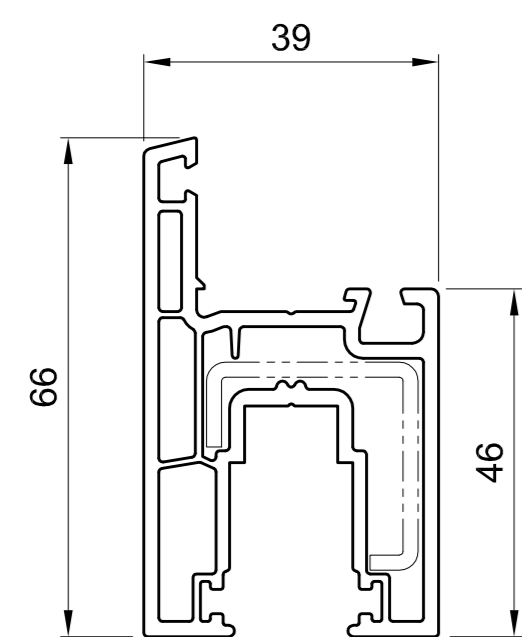
651 010 Reinforcement 28x27,5: 655 210
