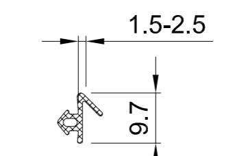
414 010 Glazing gasket for frame / casement / mullion
