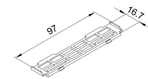
657 040 Glazing bridge
