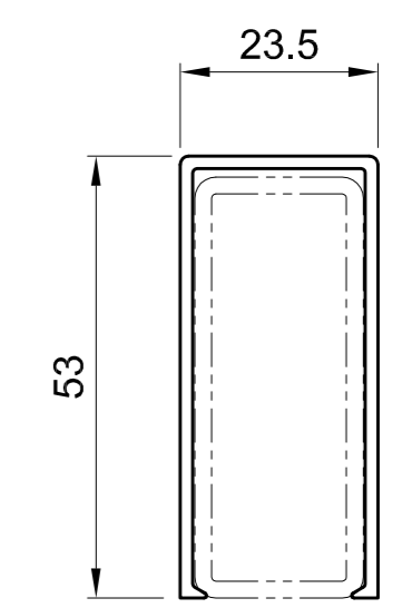
656 330 Steel tube 20x50: 655 030
