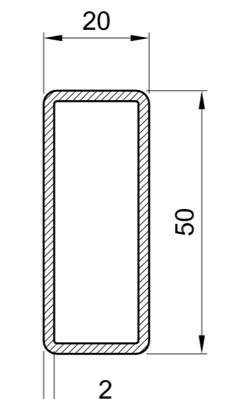
655 030 20 / 50 / 2 mm galvanized steel Ix= 7,55 cm 4 Iy= 1,72 cm 4 Insert: 656 330
