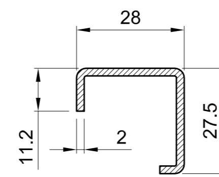
655 210 28 / 27,5 / 2 mm galvanized steel Ix= 1,03 cm 4 Iy= 1,37 cm 4 Insert: 650 010
