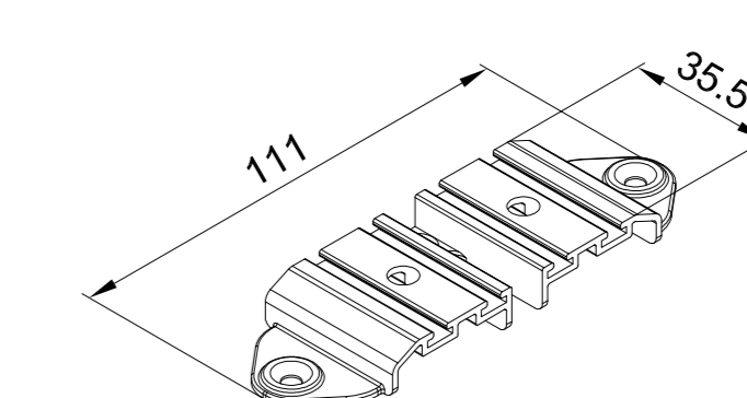
657 020 Sealing bridge
