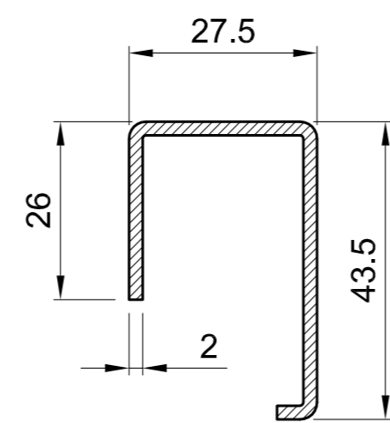
655 230 27,5 / 43,5 / 2 mm galvanized steel Ix= 3,43 cm 4 Iy= 2,35 cm 4 Insert: 651 030
