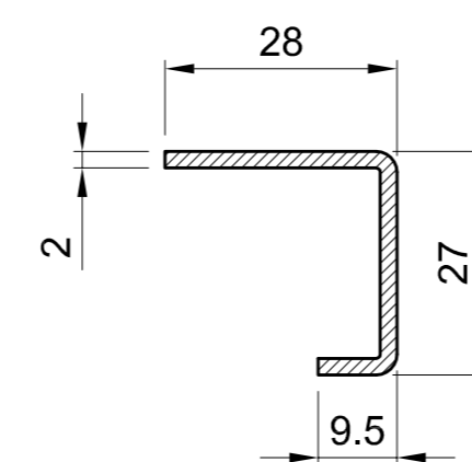
655 250 28 / 27 / 2 mm galvanized steel Ix= 1,15 cm 4 Iy= 0,81 cm 4 Insert: 651 050
