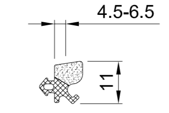
414 573 Glazing gasket foamed for frame / casement / mullion
