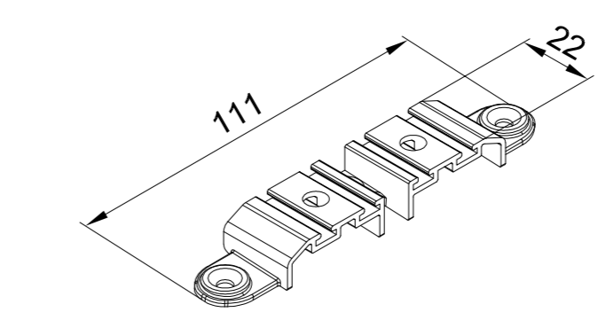
657 030 Sealing bridge
