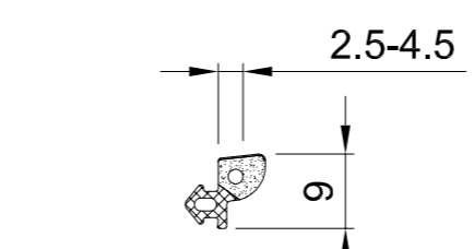
414 566 Glazing gasket for frame / casement / mullion
