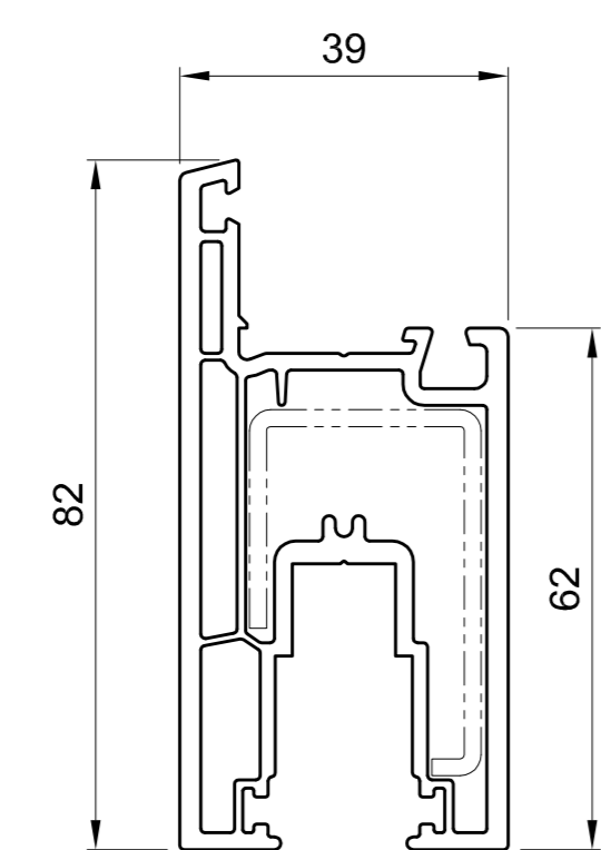
651 030 Reinforcement 27,5x43,5: 655 230
