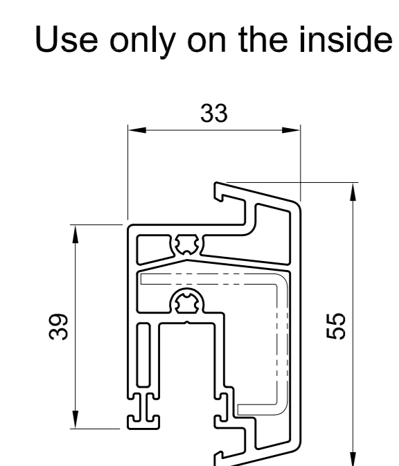
651 050 Reinforcement 28x27: 655 250
